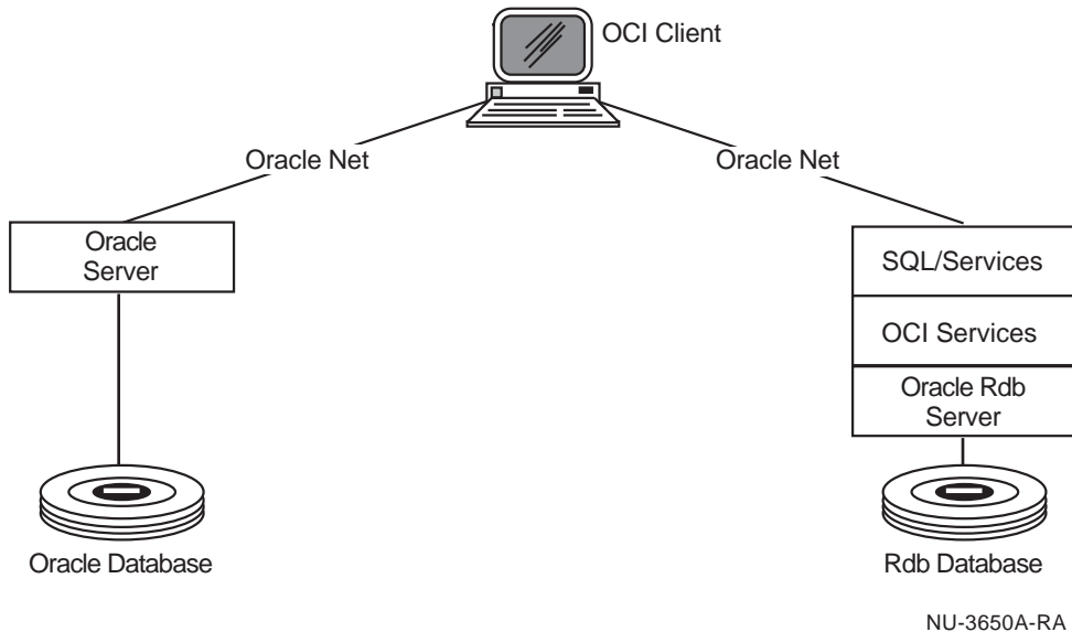
Figure 1–4 Client/Server Processing
